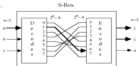
Fig 2.1 Substitution Operation
