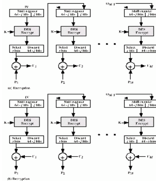
Figure 3.14 1-bit Output Feedback (OFB) Mode
