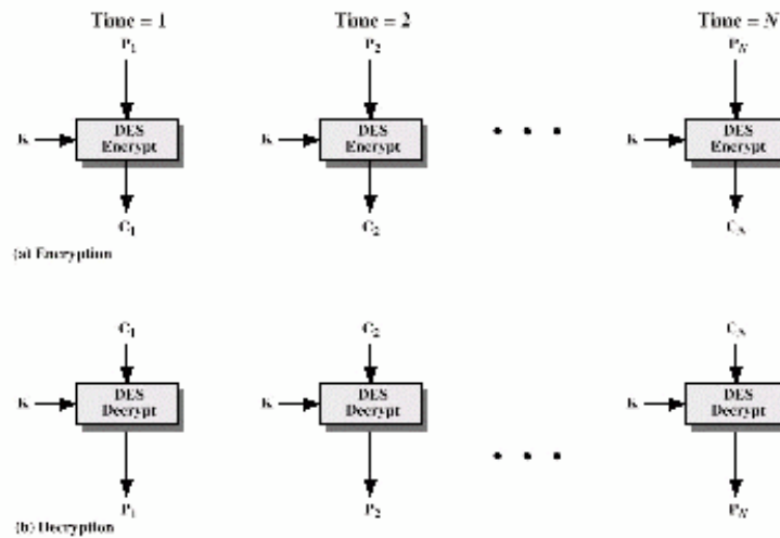
Figure 3.11 Electronic Codebook (ECB) Mode
