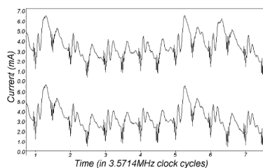
Figure 3: SPA trace showing individual clock cycles.
