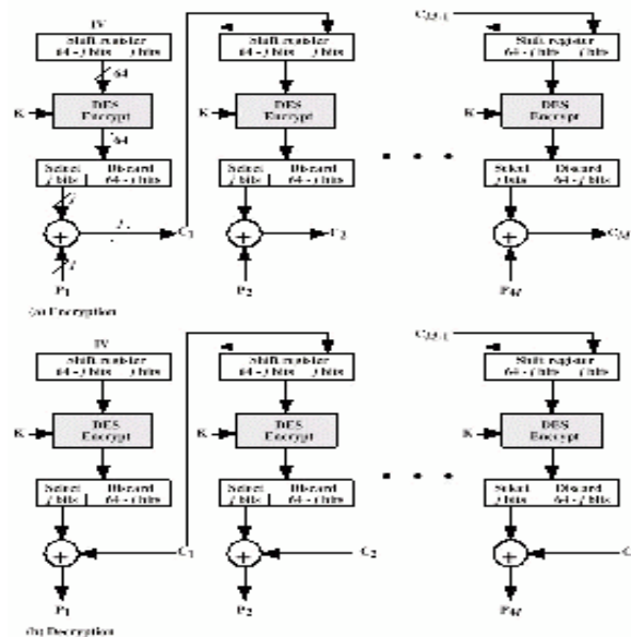
Figure 3.13 J-Bit Cipher Feedback (CFB) Mode
