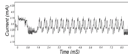
Figure 1: SPA trace showing an entire DES operation.
